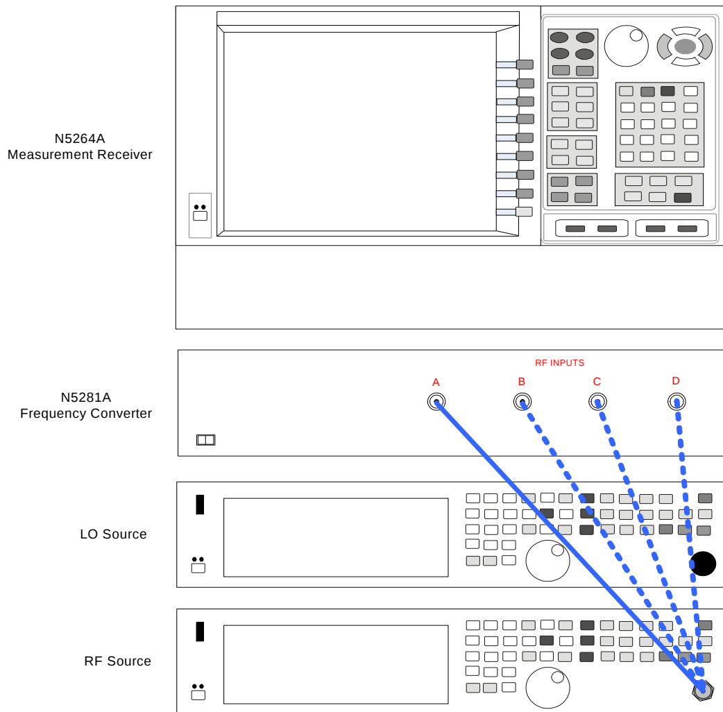
Figure 14 Front Panel N5281A and N5264A without Option 108
